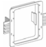
1 gang p-ring 2.5" W x 4.25" H x 1.5" D (63.5 x 108 x 38.1 mm) 7200-119576: CADMP1P Shipping Weight 1oz (.05kg)
